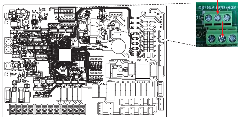
Innen-PCB
