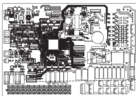
Innen-PCB
