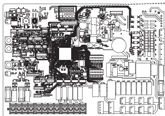
Innen-PCB
